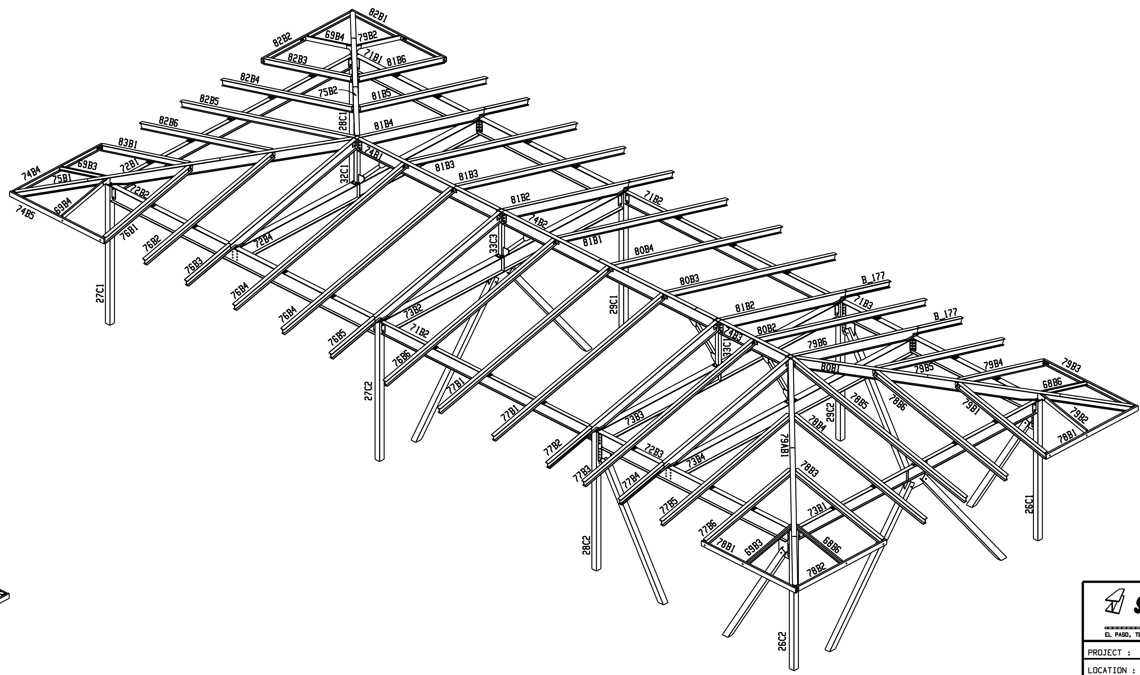
3D ISOMETRIC VIEW ( @ HIGH ROOF LEVEL )
